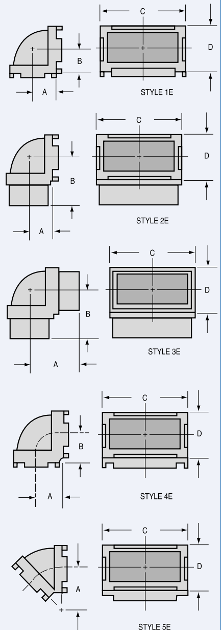
WAVEGUIDE BENDS
